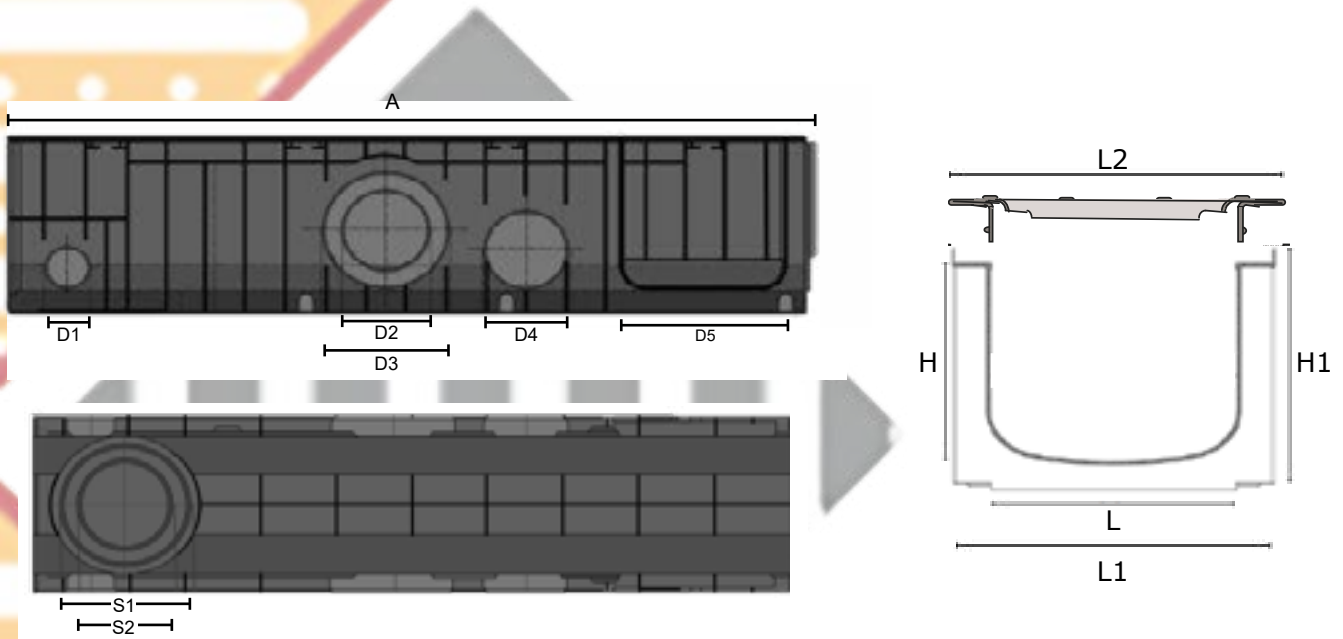
SABDRAIN 951/952
